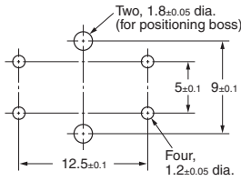
PCB Mounting (Top View) (Single-sided PCB, t=1.6)
