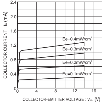
Fig.2 Output characteristics
