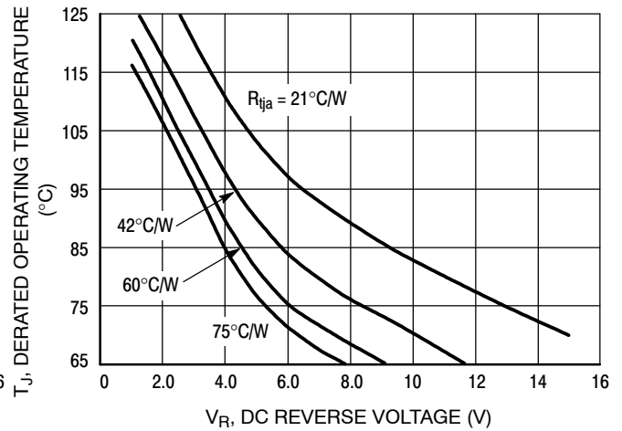
Figure 8. Typical Operating Temperature Derating Per Leg*
