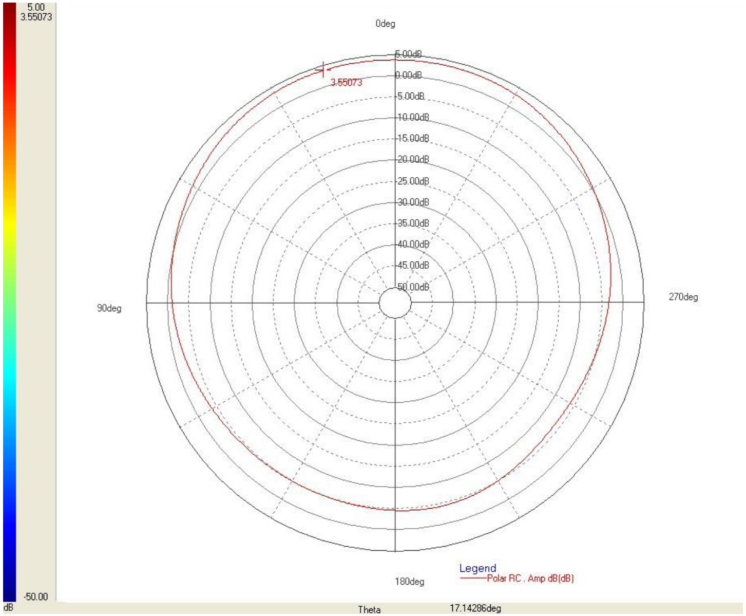
Radiation Pattern in XZ plane
